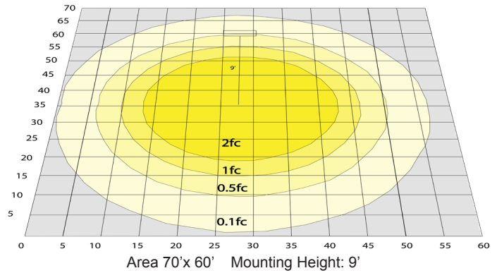
Area 70'x 60' Mounting Height: 9'
